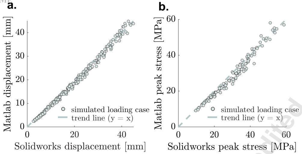
Fig. 9. Displacements at the CoP (a) and maximum von Mises stress (b) of prosthetic foot models under load; calculated with SOLIDWORKS and the MATLAB constitutive model (FEA).
