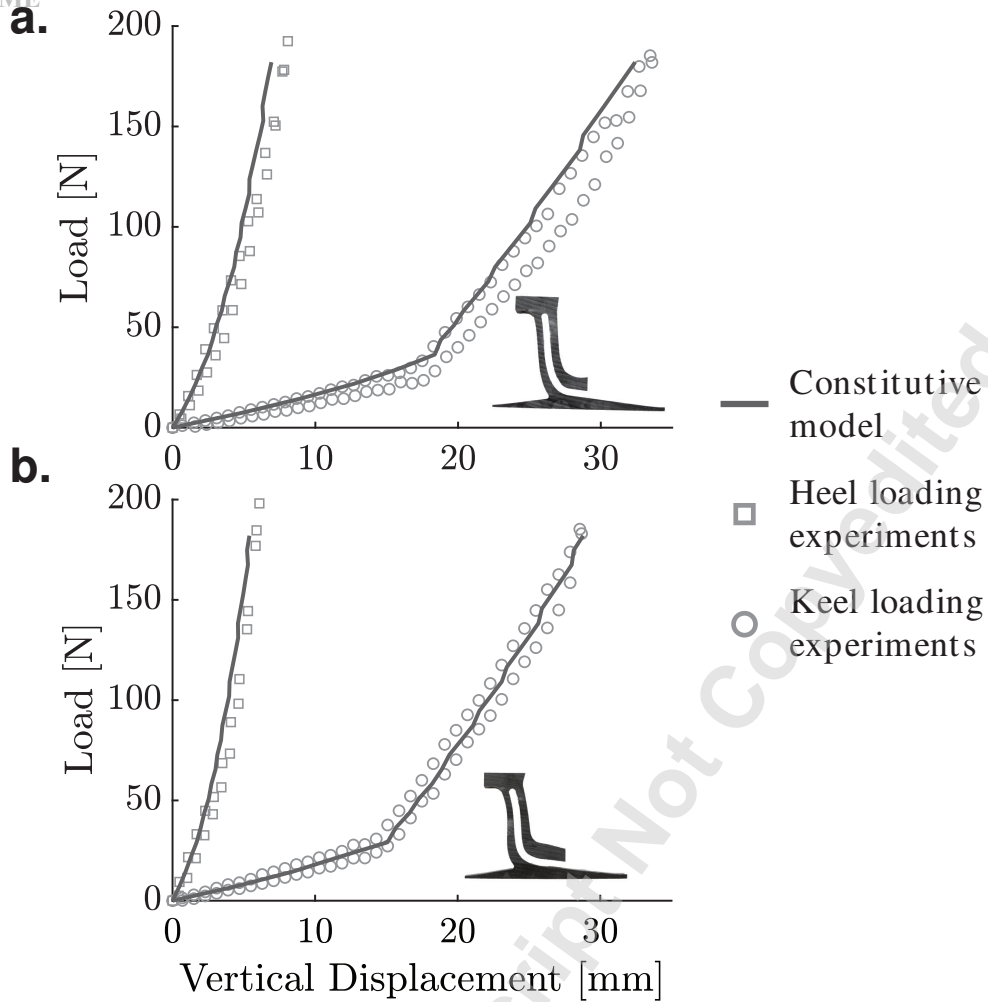
Fig. 7. Load-displacement curves for the two multi-keel prosthetic foot prototypes (a, b) measured with the Instron machine and compared with the constitutive model results. The prototypes were tested at the heel ( CoP_{heel} = -30 \pm 0.1 mm) and at the keel ( CoP_{keel} = 130 \pm 0.1 mm). Prototype a corresponds to a 60 kg user, and prototype b to an 80 kg user.
