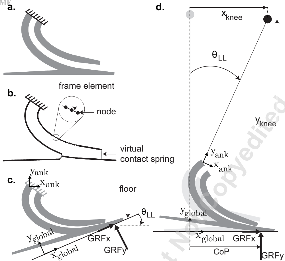
Fig. 3. Multi-keel constitutive model. a) Multi-keel prosthetic foot model defined by the set of 15 design variables (Fig. 2a). b) Finite-element model, based on frame elements, of the multi-keel foot with the virtual contact spring that enforces the non penetration contact condition between the two keels once contact is detected. c) Deformed shape of the multi-keel foot in the ankle reference frame under a set of GRFs applied at a CoP. d) Lower leg orientation and knee position in the global frame resulting from the deformation of the prosthetic foot. The undeformed shape (light grey) is overlaid with the deformed shape (dark grey) of the prosthetic foot.
