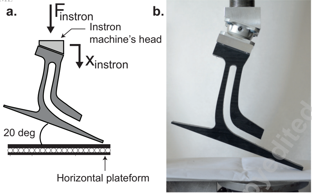
Fig. 6. ISO ultimate static tests experimental setup. a) Schematic of the experimental setup and b) photograph of a prototype prosthetic foot being loaded on the Instron machine.
