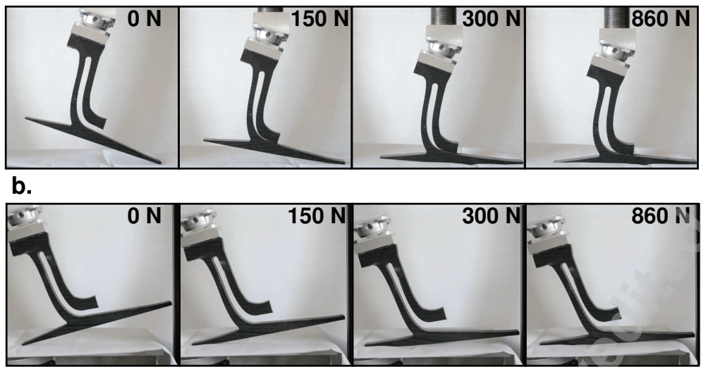
Fig. 8. Multi-keel prosthetic foot tested under the ISO ultimate static loading cases in the Instron machine, (a) corresponds to the forefoot loading and (b) to the heel loading scenario. The prosthetic foot shown here corresponds to the 60 kg user design.
