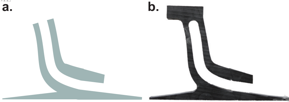
Fig. 4. Multi-keel foot architecture. a) Parametric model of a multi-keel foot. b) Physical embodiment of a multi-keel foot.
