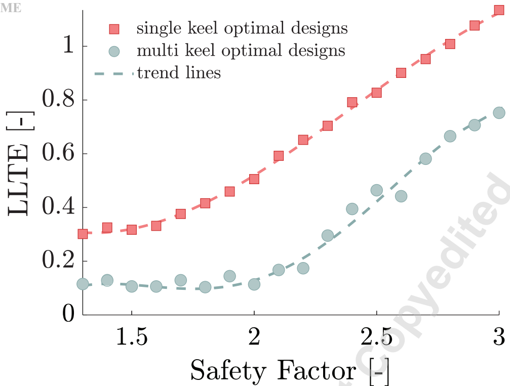
Fig. 10. LLTE values of single-keel (square markers) and multi-keel (round markers) feet optimized for level-ground walking at comfortable speed for safety factors ranging from 1.3 to 3. The dashed lines are the 4th order polynomial fit representing the trend between optimal LLTE value and safety factor constraint for both foot architectures.
