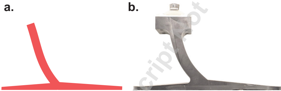
Fig. 1. Single-keel foot architecture. a) Parametric model of a single-keel foot. b) Physical embodiment of a single-keel foot.
