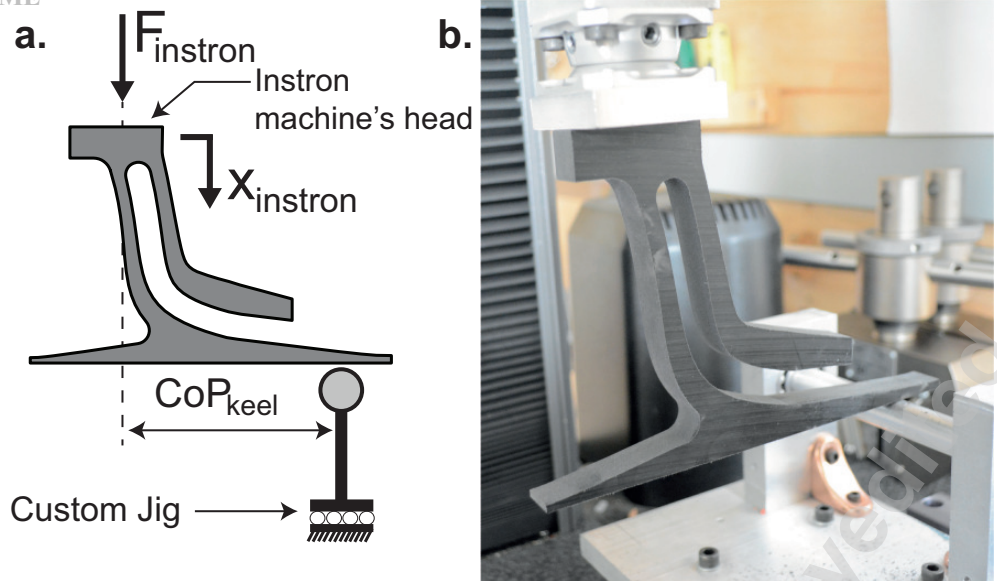
Fig. 5. Mechanical tests experimental setup. a) Schematic of the experimental setup and b) photograph of a prototype prosthetic foot being loaded on the Instron machine.
